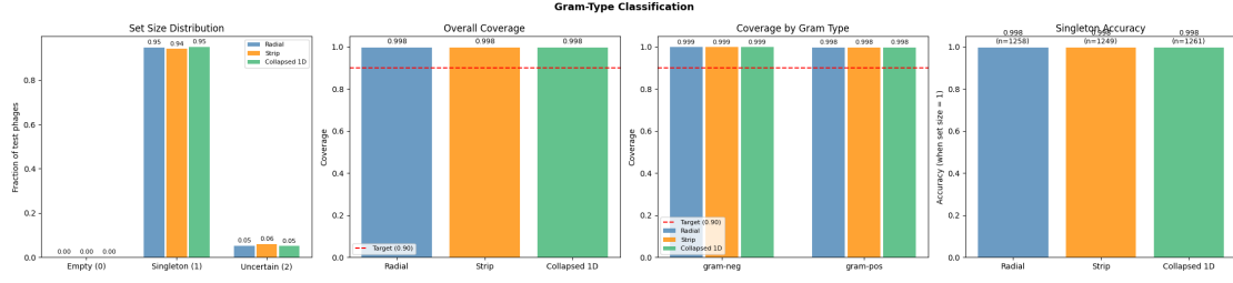
Figure 5.1: Gram type classification performance across Radial, Strip, and Collapsed 1D geometries on the test split (Fold 0, nominal target 1 - \alpha = 0.90 ). Panels show (left to right): prediction set size distribution, marginal empirical coverage, class-conditional coverage, and singleton accuracy with sample counts ( n ).
